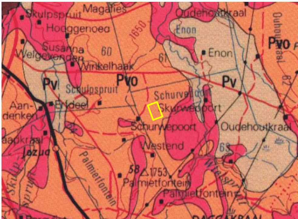
Figure 5: Geological map of the area around the Farm Schurvepoort with the site for the Renewstable® Qhakaza hydrogen plant indicated within the yellow rectangle. Abbreviations of the rock types are explained in Table 2. Map enlarged from the Geological Survey 1: 250 000 map 2726 Frankfurt.
